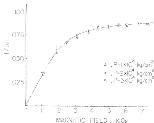
Fig. 3. Field dependence of normalized magnetization that was induced by squeezing, measured at -196^\circ\text{C} . Solid curve represents the most favorable Langevin function. I_0 s are taken as 5.62, 3.32 and 1.80 emu/g for applied pressures of 1 \times 10^4 , 2 \times 10^4 and 3 \times 10^4 Kg/cm 2 , respectively.
